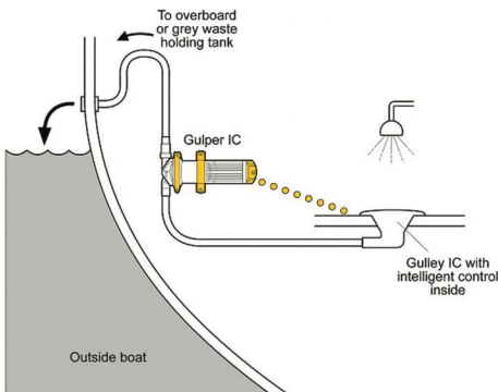
TYPICAL INSTALLATION
