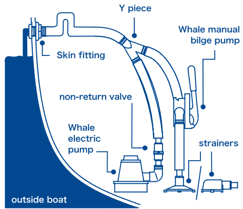
TYPICAL INSTALLATION
