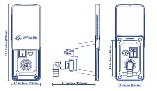
4 IN 1 FITTING
