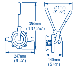
Bulkhead/Removable Handle BP9021
