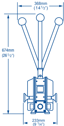
BP3000 SIDE VIEW
