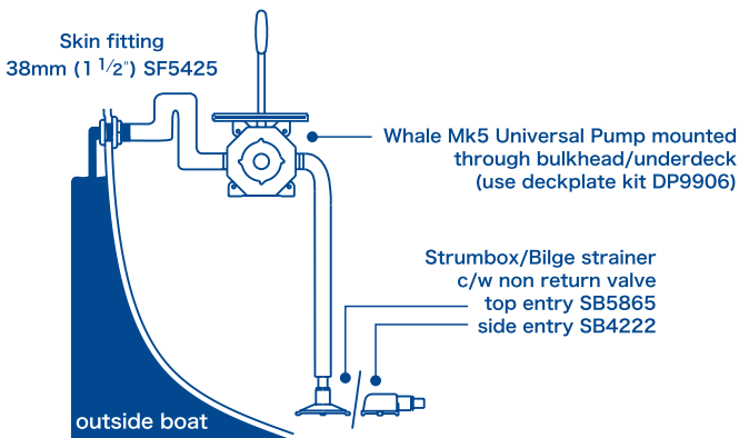
TYPICAL INSTALLATION
